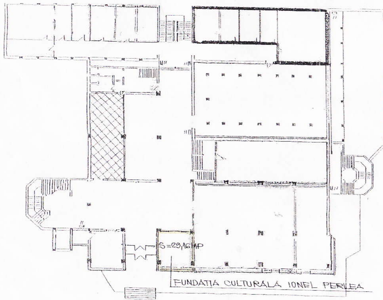
PLAN PARTER
